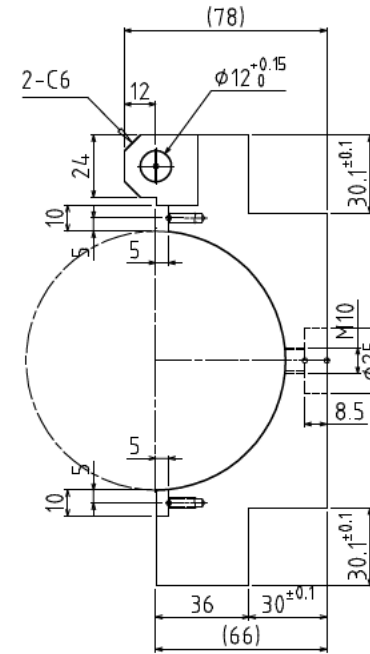
B-B SECTION
